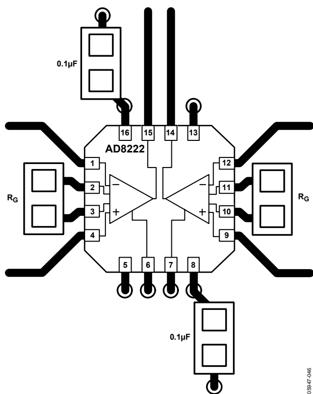
Figure 46. Example Layout
